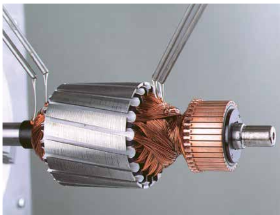
An impregnation resin applied by trickling
